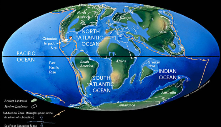
K/T Boundary 66 Ma
