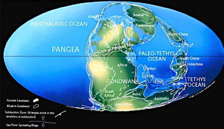
Early Jurassic 195 Ma
