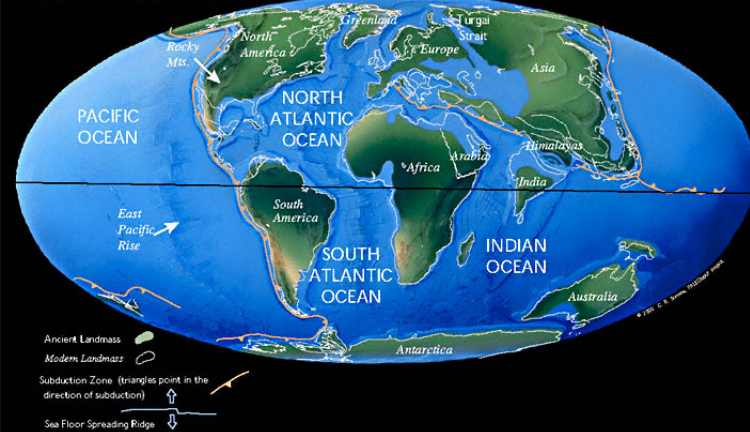
Middle Eocene 50.2 Ma
