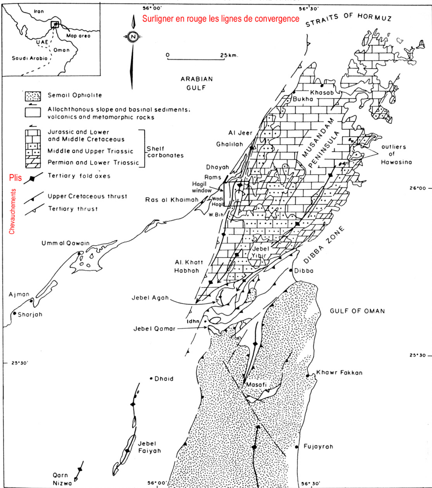
Geologic map of the Musandam Peninsula and Dibba zone, United Arab Emirates.
